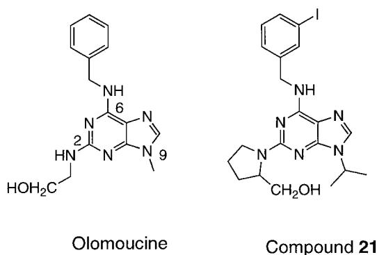
Scheme 1. Chemical structure of olomoucine and compound 21 .
