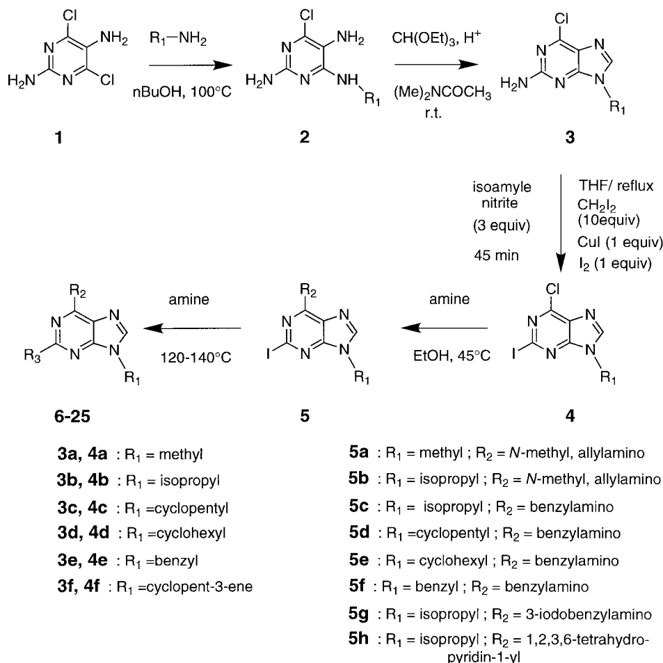
Scheme 2. General pathways for the synthesis of the 2,6,9-trisubstituted purines in the series reported herein.
